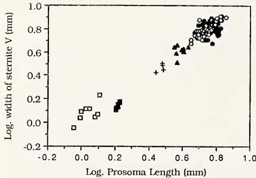
Figure 1.—A log-log bivariate morphometric plot, showing the 5 juvenile instars in the scorpion, Euscorpis flavicaudis ( N = 163 ). Instars determined either by morphological differences (e.g., first and second instars) or cluster statistics (adults and fifth instars). White squares = first instar; black squares = second; cross = fourth; black triangle = fifth; white circle = adult females; black circle = adult males. Regression equation of this relationship (including all instars other than 1st): y = 1.139x - 0.079 , R^2 = 0.974 , N = 155 .
